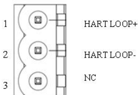
HART Channel 1
